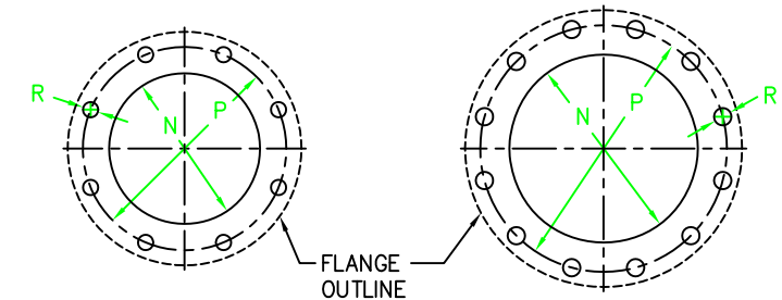
TANK CUT FOR TPS 50, TPS 80 AND TPS 100
